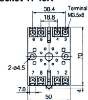
Socket TP48X
